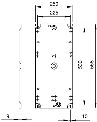
Mounting plates
